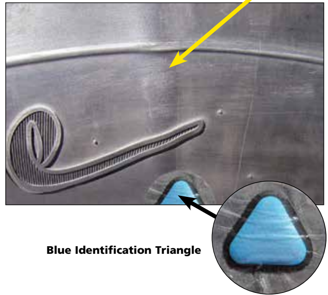
Acceptable Bulges \frac{3}{8} " or Less
