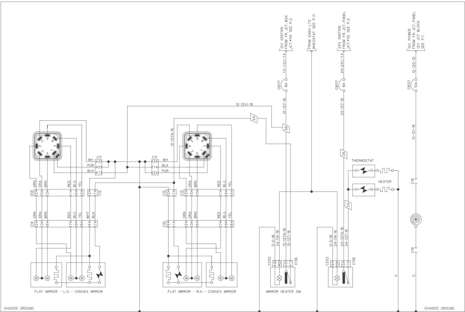
REAR VIEW MIRROR - ADJUSTMENT & HEATER SW. (RAMCO) | MIRROR (IKI) | CIGAR LIGHTER
