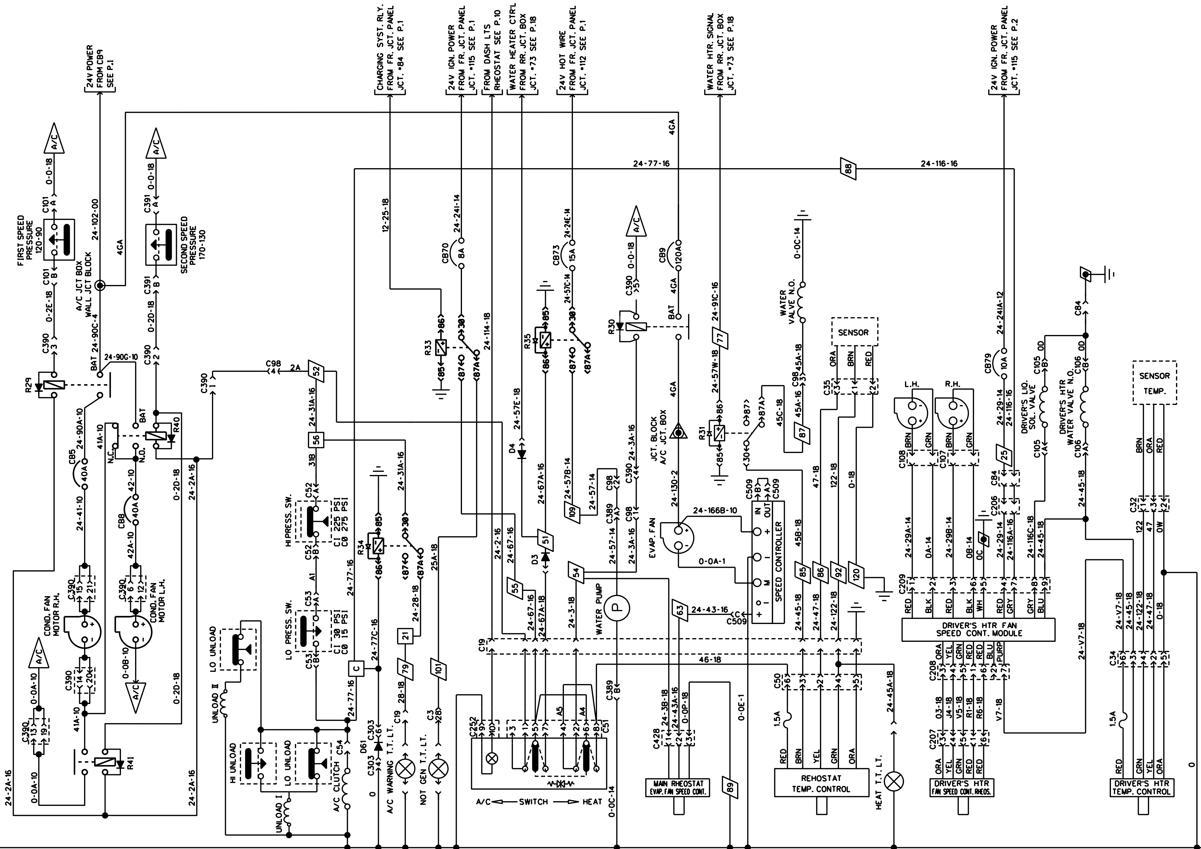
A/C AND HEAT SYSTEM (FULL AIR)
