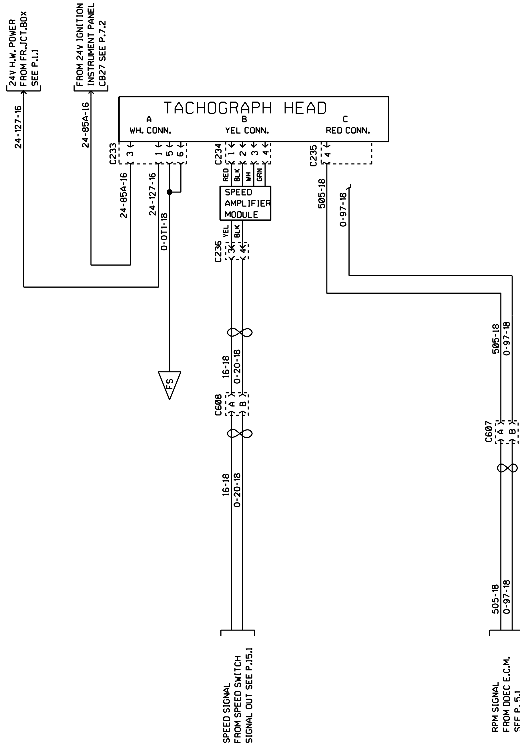
ELECTRONIC TACHOGRAPH
