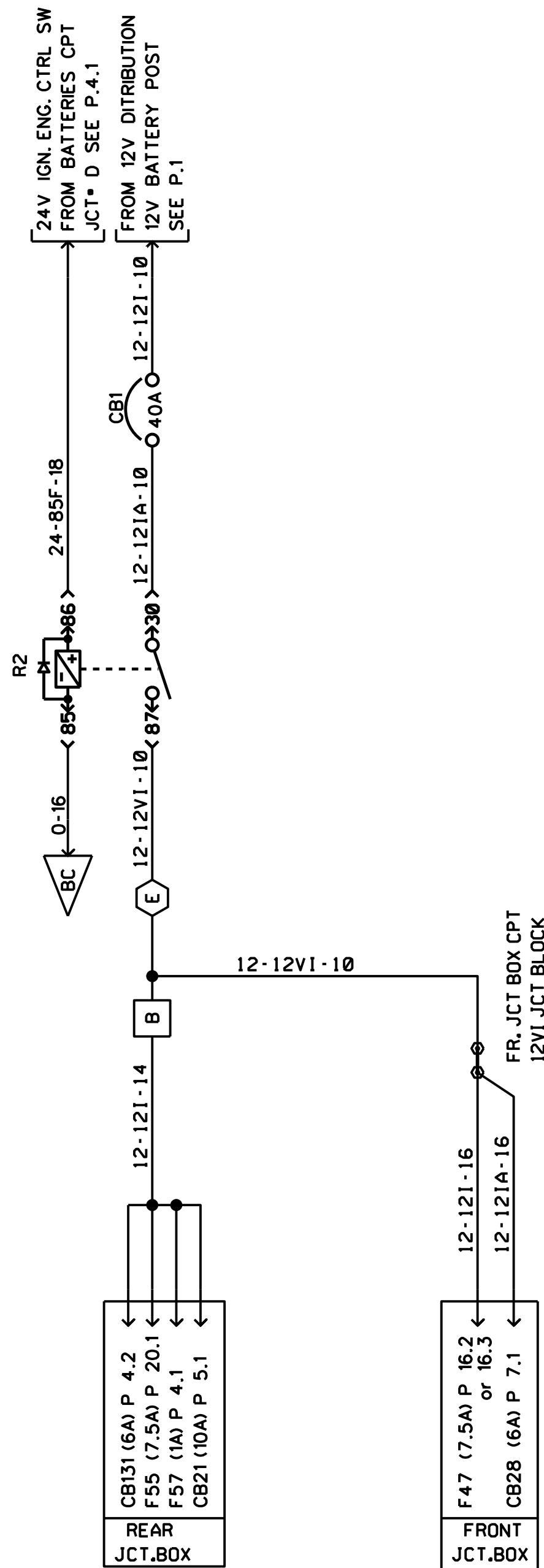
12V IGNITION
