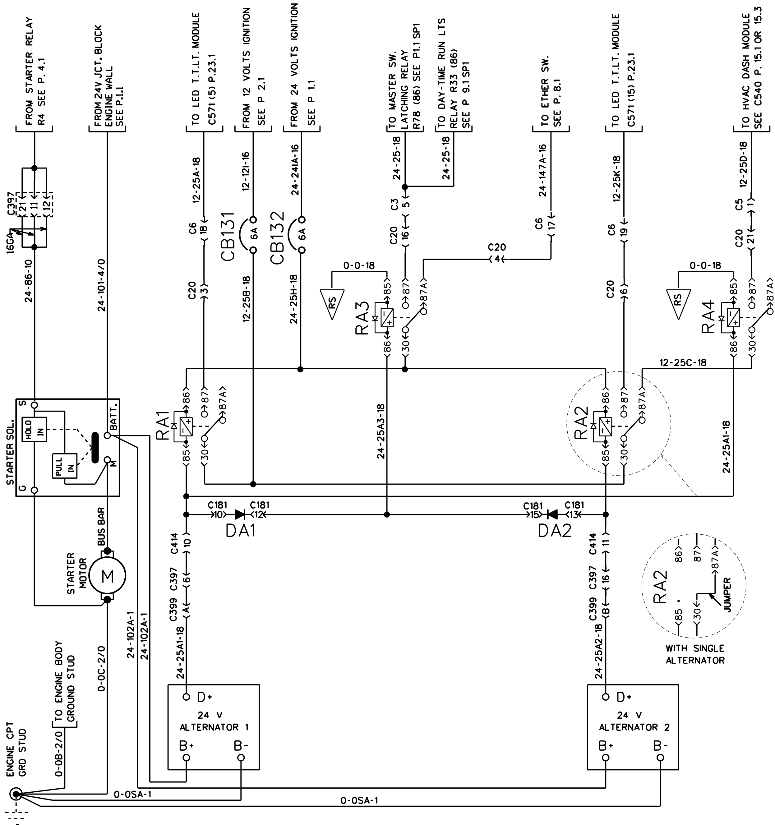
STARTER & ALTERNATOR BOSCH
