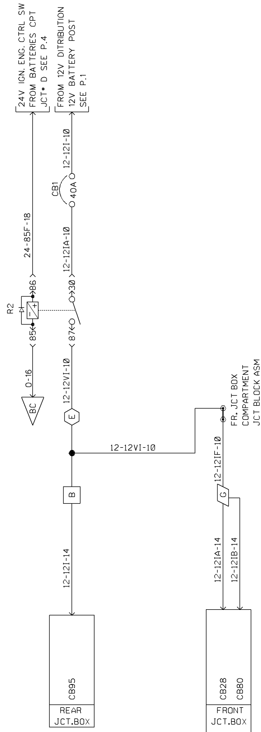
12V IGNITION
