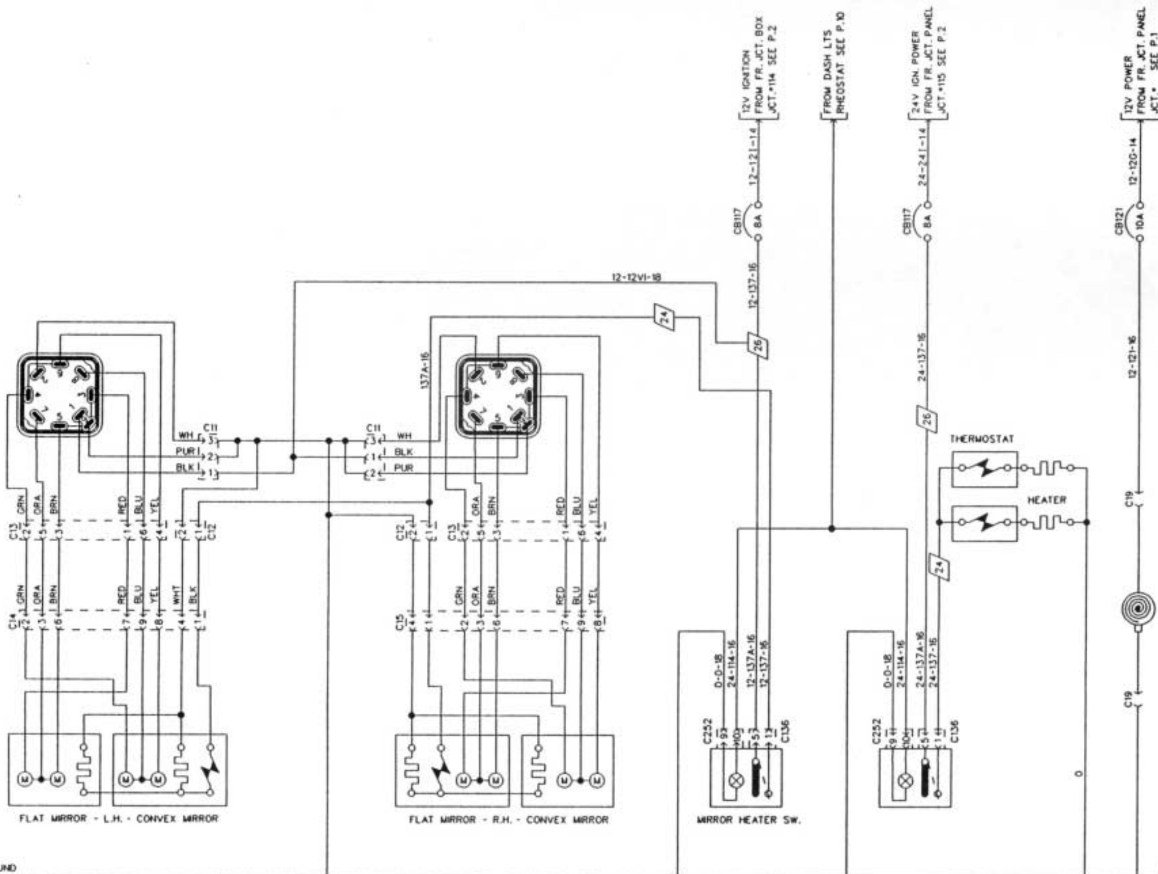
REAR VIEW MIRROR - ADJUSTMENT & HEATER SW.
